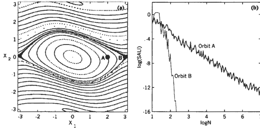
Fig. 1. (a) Phase plot of the 2D map (8) for \nu = 0.5 . The initial conditions of the ordered orbit A ( x_1 = 2, x_2 = 0 ) and the chaotic orbit B ( x_1 = 3, x_2 = 0 ) are marked by black and light-gray filled circles respectively. (b) The evolution of the SALI, with respect to the number N of iterations of the 2D map (8) for orbit A (black line) and for orbit B (gray line).
