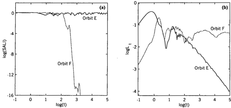
Fig. 4. The evolution in log-log scale of (a) the SALI and (b) the finite time Lyapunov characteristic number L_t as a function of time t , for the Hamiltonian (10) with H=1/8 , for the ordered orbit E with initial condition x = 0 , y = 0.55 , p_x \simeq 0.2417 , p_y = 0 (black line) and for the chaotic orbit F with initial condition x = 0 , y = -0.016 , p_x \simeq 0.49974 , p_y = 0 (gray line).
