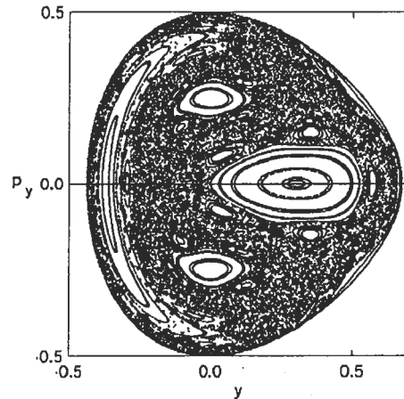
Fig. 3. The Poincaré surface of section for x = 0 of the two degrees of freedom Hénon-Heiles Hamiltonian (10) for H=1/8 . The projection on the PSS of the initial conditions of the ordered orbit E ( x = 0 , y = 0.55 , p_x \simeq 0.2417 , p_y = 0 ) and the chaotic orbit F ( x = 0 , y = -0.016 , p_x \simeq 0.49974 , p_y = 0 ) are marked by black and light-gray filled circles respectively. The axis p_y = 0 is also plotted.
