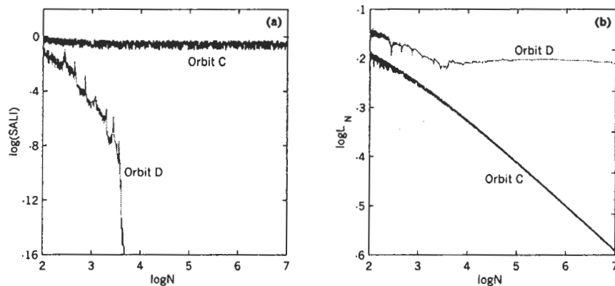
Fig. 2. The evolution in log-log scale of (a) the SALI and (b) the finite time Lyapunov characteristic number L_N , with respect to the number N of iterations of the 4D map (9) with \nu = 0.5 , \kappa = 0.1 , \mu = 10^{-3} , for the ordered orbit C with initial condition x_1 = 0.5 , x_2 = 0 , x_3 = 0.5 , x_4 = 0 (black line) and for the chaotic orbit D with initial condition x_1 = 3 , x_2 = 0 , x_3 = 0.5 , x_4 = 0 (gray line).
