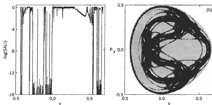
Fig. 5. (a) The value of SALI for t = 4,000 for orbits with initial conditions on the p_y = 0 axis of the PSS shown in figure 3, as a function of the y variable of the initial condition. The data are plotted as black points and are connected by gray lines. (b) Regions of different values of the SALI on the PSS (y, p_y) after 1,000 time steps. Initial conditions that give \text{SALI} < 10^{-12} are marked by black points, initial conditions that give 10^{-12} \leq \text{SALI} < 10^{-8} are marked by deep gray points, initial conditions that give 10^{-8} \leq \text{SALI} < 10^{-4} are marked by gray points, while initial conditions that give 10^{-4} \leq \text{SALI} are marked by light gray points.
